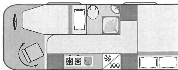
DAYTIME LAYOUT
